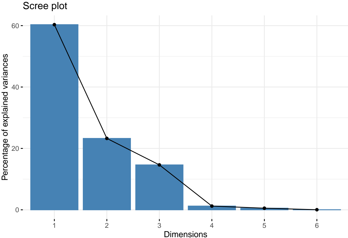
Part of variance explained by each dimension of the PCA projection.
